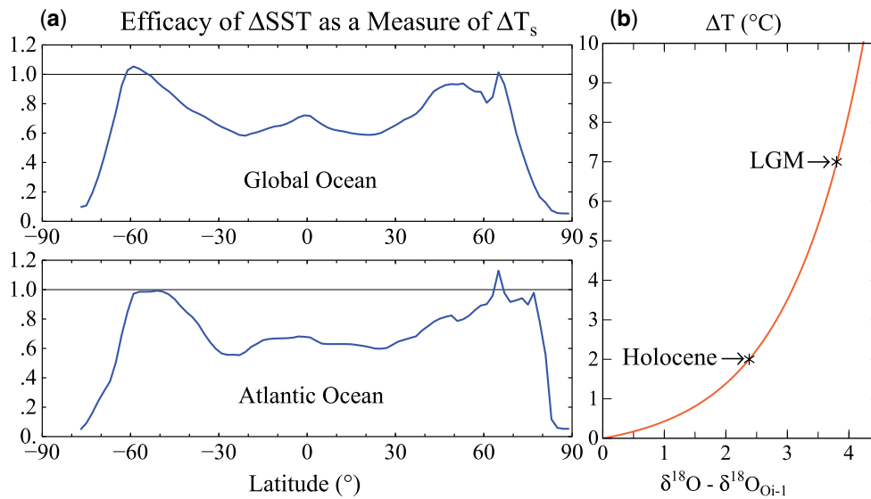
Figure 7. (a) Ratio of \Delta SST (latitude) to global T_S change for all ocean and the Atlantic Ocean, based on equilibrium response (years 4001–4500) in 2 \times CO_2 simulations of GISS (2020) model. (b) \Delta T , the amount by which T_S change exceeds T_{do} change, based on an exponential fit to the two data points provided by the Holocene and LGM (see text).
